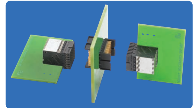
ORTHOGONAL MIDPLANE
