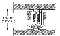
SURFACE-MOUNT RECEPTACLE TO 6.42 mm (0.253 in.) TALL SURFACE-MOUNT HEADER
