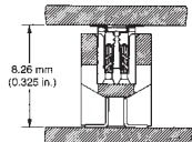
SURFACE-MOUNT RECEPTACLE TO 8.25 mm (0.325 in.) TALL SURFACE-MOUNT HEADER
